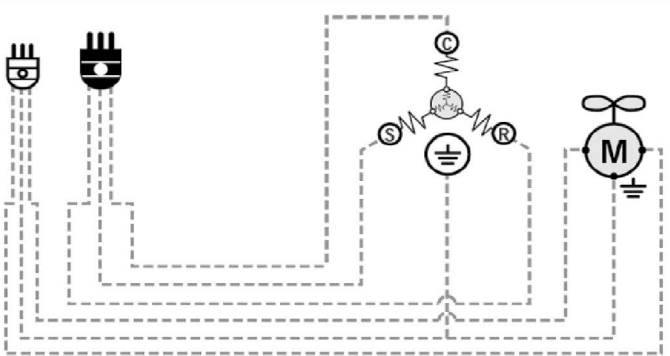
Compressor Terminals C = Common R = Run S = Start
