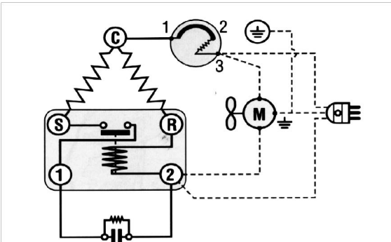
Compressor Terminals C = Common R = Run S = Start
