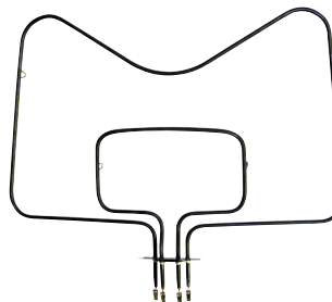
37-UB820 - Whirlpool 9750417 1100/2500W, 250V, 20 1/2"W×15 3/4"L, 2 1/2" Inserts
