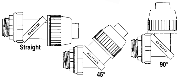
One SwivelLok™ Connector Fits Any Position
